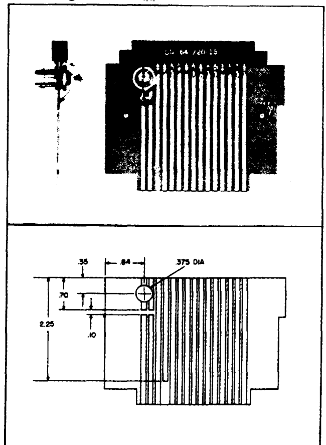
Figure 5-1. Type 1 Extender Board
