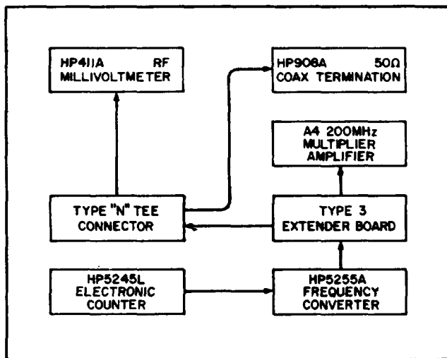
Figure 5-6. 200 MHz Multiplier/Amplifier Test Setup
